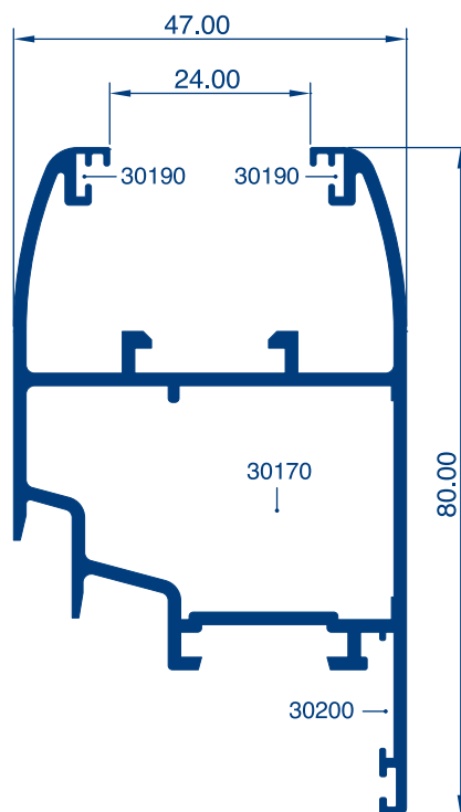
Ref. 2007 Espesor 1.5
